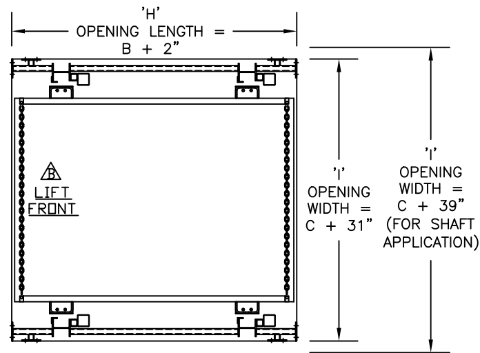
PLAN VIEW - UPPER LEVEL
