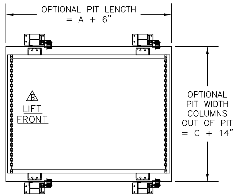
△ PLAN VIEW - LOWER LEVEL
