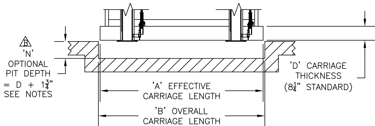
△ LIFT FRONT VIEW
