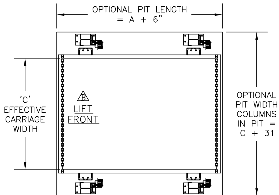
△ PLAN VIEW - LOWER LEVEL
