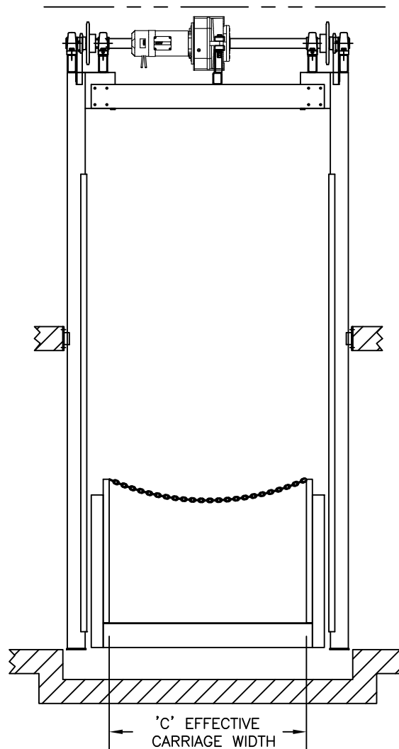
LIFT FRONT VIEW
