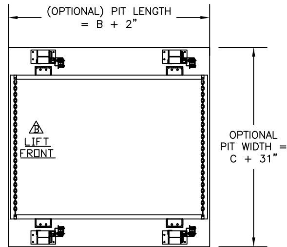
PLAN VIEW - LOWER LEVEL
