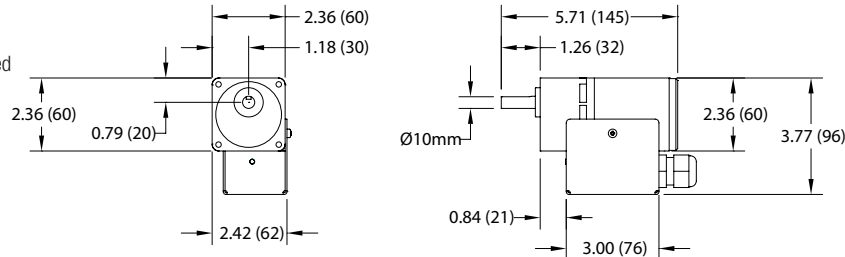
Chart 1 Parallel Shaft
