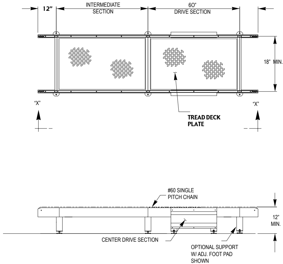
SECTION X-X
