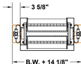
Section A-A w/ Optional T-Slot Take-Up Brg.
