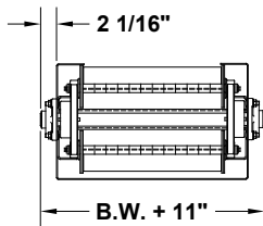
Section A-A w/ Std. 4 Bolt Flange Brg.
